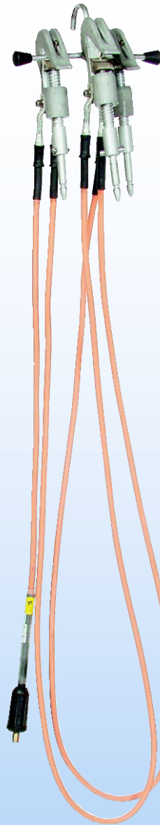
3-Phase Earthing Device JSKL3-STG Line length: 1,0+2,5+2,5 m
